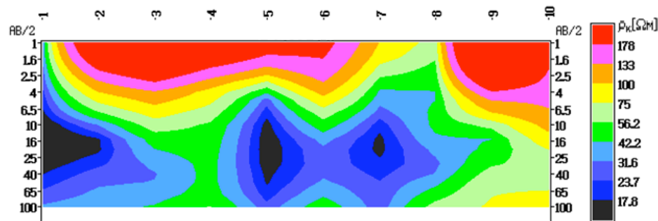
Fig. (4). Pseudosection of the profile Z.
