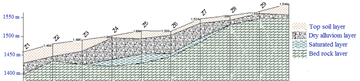
Fig. (4). Pseudosection of the profile Z.
