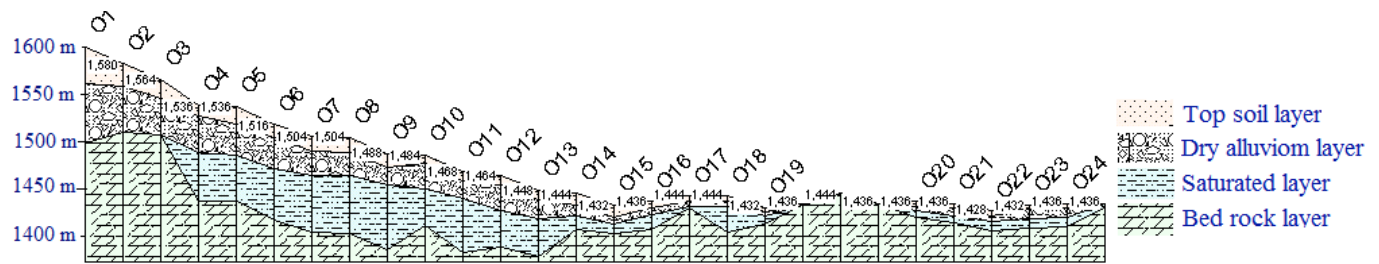
Fig. (7). Geoelectric section of profile O.
