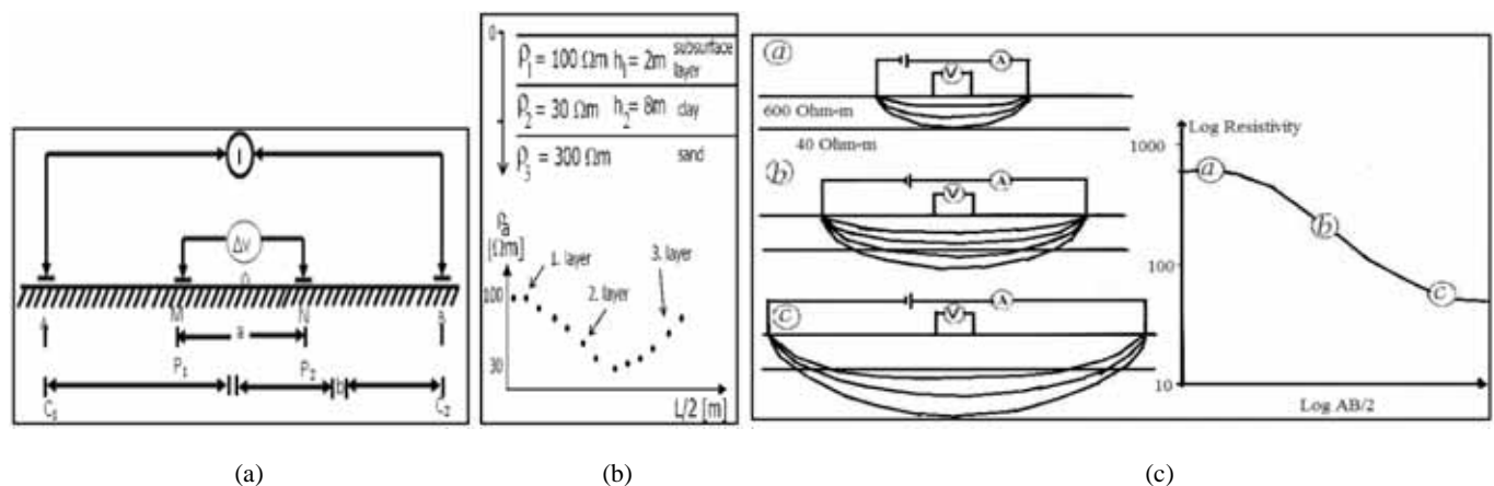
Fig. (2). VES geoelectric sounding (a) Schlumberger array. Current is delivered through the electrodes A and B, and voltage readings are made with electrodes M and N, (b) A Schlumberger sounding curve in a simple three-layer system. The apparent resistivity is plotted versus the AB/2 , (c) As the distance between the current electrodes is increased, so the depth to which the current penetrates is increased.
