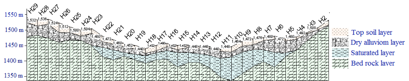
Fig. (6). Geoelectric section of profile H.
